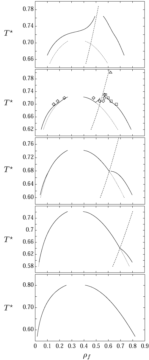
Fig. 2. Variation of \alpha of the phase diagram of the binary symmetric bulk mixture from MSA: \alpha = 0.65, 0.70, 0.75, 0.80 , and 0.90 (from top to bottom); full line: G-L, G-DF, or L-DF coexistence curves; dotted line: metastable G-L transition; dashed line: \lambda -line; symbols: grand canonical Monte Carlo simulations from Ref. [22]
