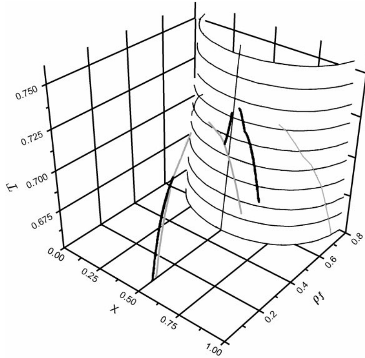
Fig. 1. Phase diagram of a binary bulk mixture in (T, \rho_f, x) -space; the curves in the (x = 1/2) plane represent the phase diagram that will be presented in the following figures (thick black and grey lines); demixing transitions are depicted for several isothermal planes by the thin grey lines in the high density regime; the critical points of this demixing transition are connected by the \lambda -line; from Ref. [23]
