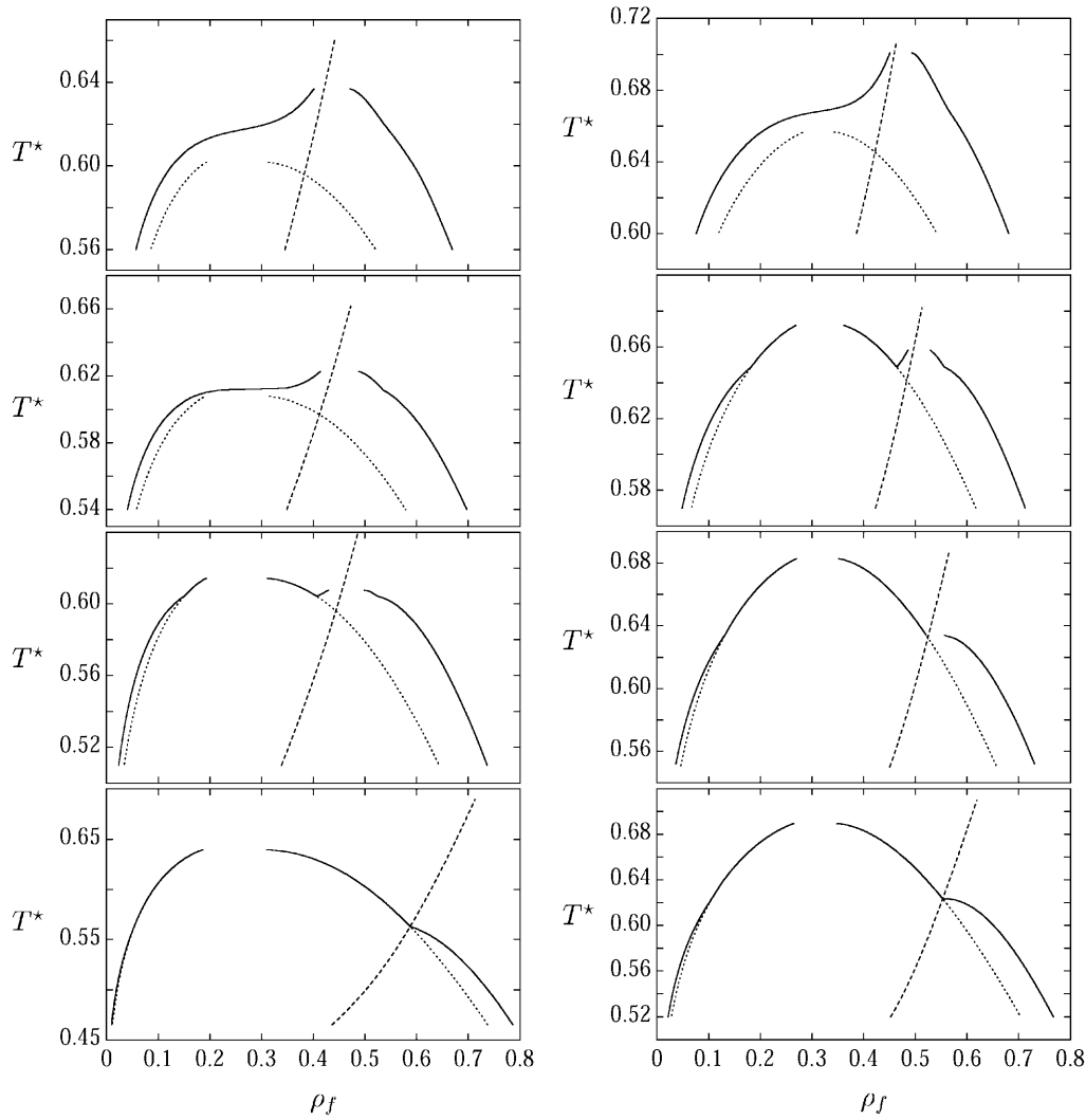
Fig. 6. Variation of the phase diagram of the binary fluid mixture in thermal equilibrium with a porous matrix from MSA with \alpha ; left column ( \rho_0 = 0.1 , y = 0 ): \alpha = 0.68, 0.70, 0.72 , and 0.80 (from top to bottom); right column ( \rho_0 = 0.1 , y = 1 ): \alpha = 0.65, 0.70, 0.73 , and 0.75 (from top to bottom); full line: G-L, G-DF or L-DF coexistence curves; dotted line: metastable G-L transition; dashed line: \lambda -line; from Ref. [22]
